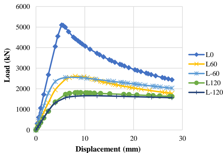
Fig. 4. Load-displacement curve of column ( H = 2 m) with different eccentricities
