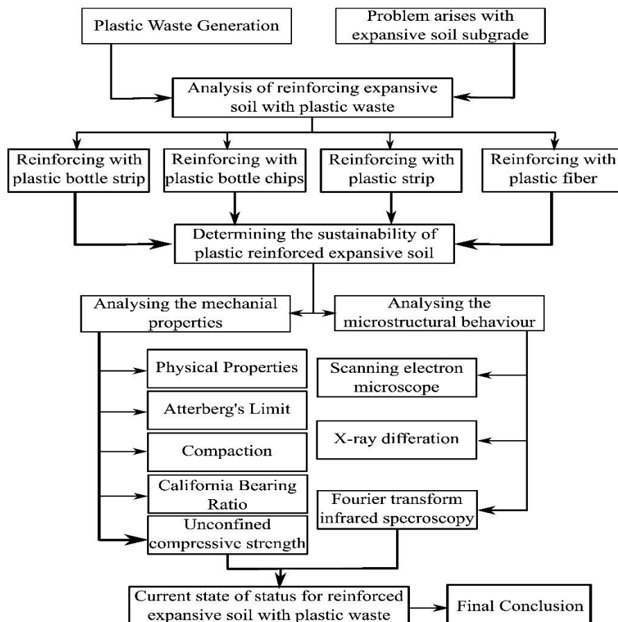
Fig. 1 Overview of stabilization of expansive soil with plastic waste
