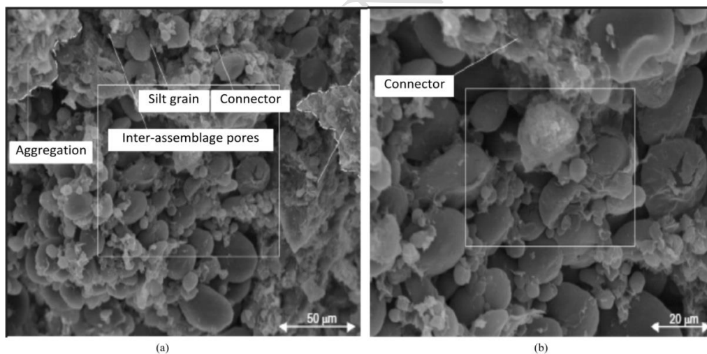
Fig. 3 Microfabric of natural soil modified from (Mirzababaei et al., 2013): (a) 500x magnification, and (b) 1000x magnification
