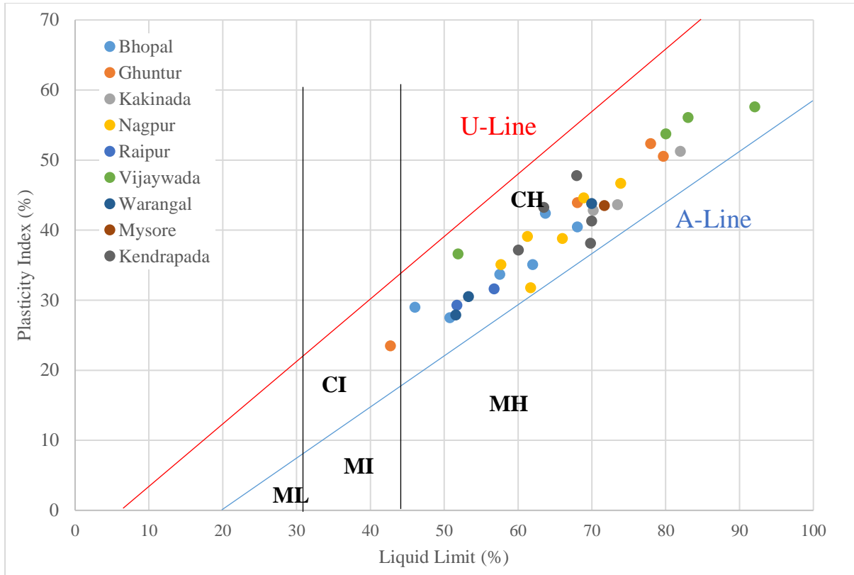
Fig. 2 Plasticity chart classification of Black cotton soil (Reddy et al., 2020)
