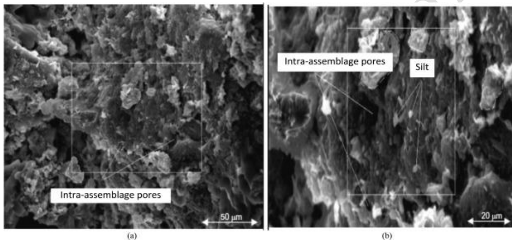
Fig. 5 Microfabric of clayey soil with 10% furan modified from (Mirzababaei et al., 2013): (a) 500× magnification, and (b) 1000× magnification
