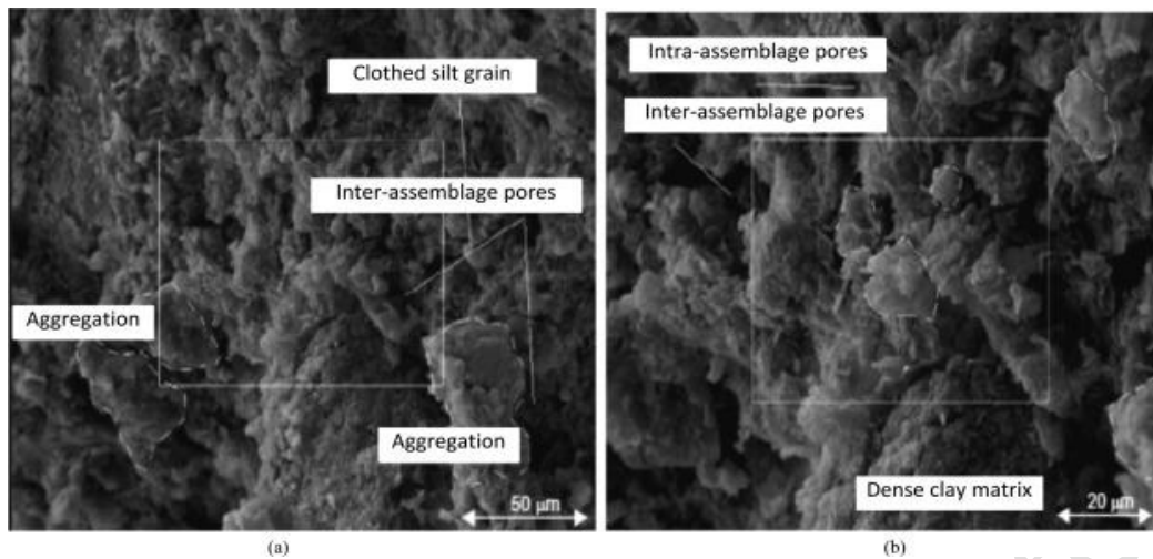
Fig. 4 Microfabric of Soil with 5% furan modified from (Mirzababaei et al., 2013): (a) 500× magnification, and (b) 1000× magnification
