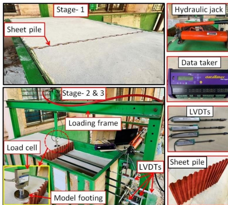
Fig. 2. Experimental test set-up
