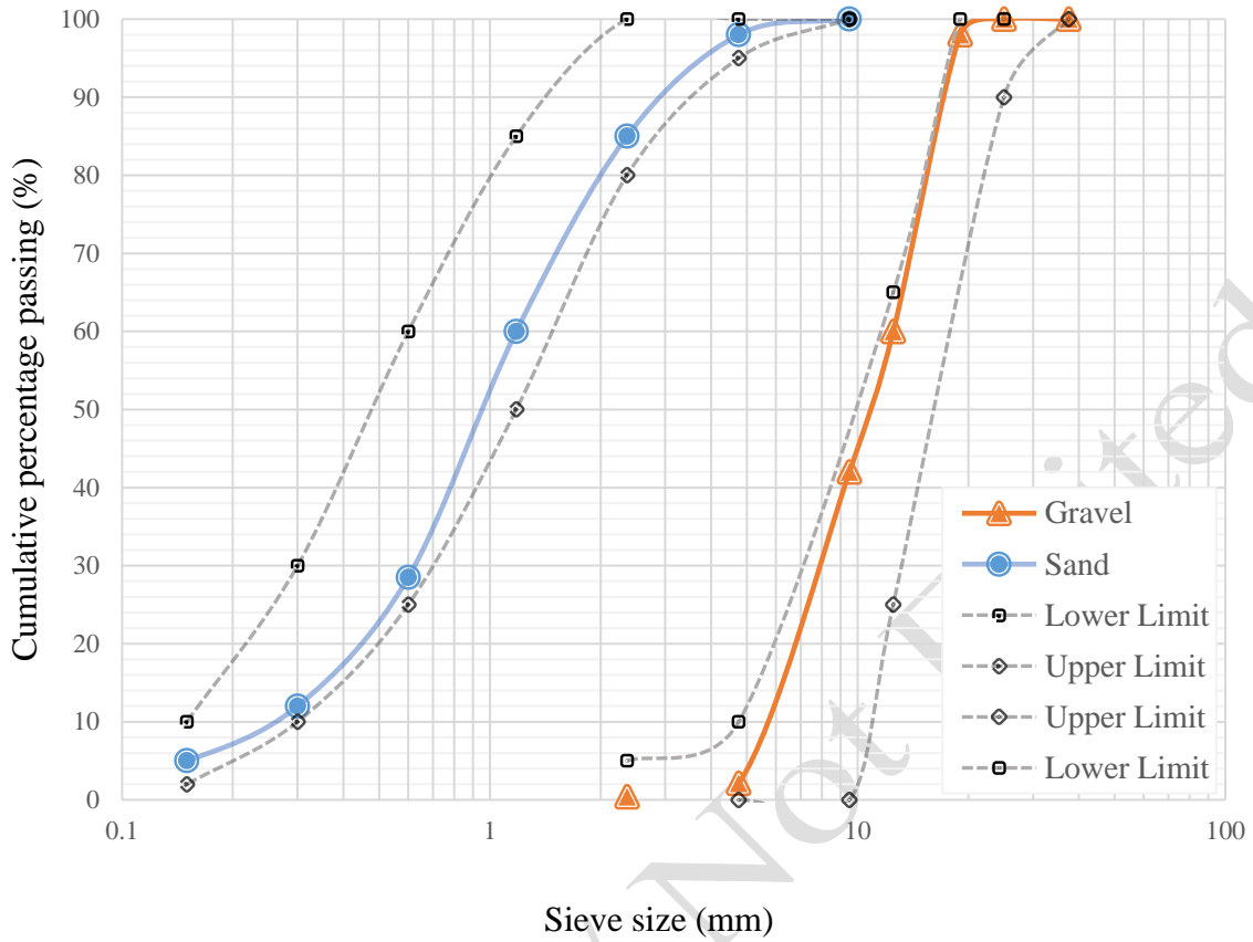
Figure 1: Granulometry curve of the materials used (sand and gravel) based on ASTM C33 standard.
