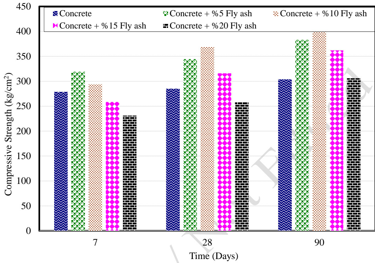
Figure 4: Changes in compressive strength of concrete samples stored in water.
