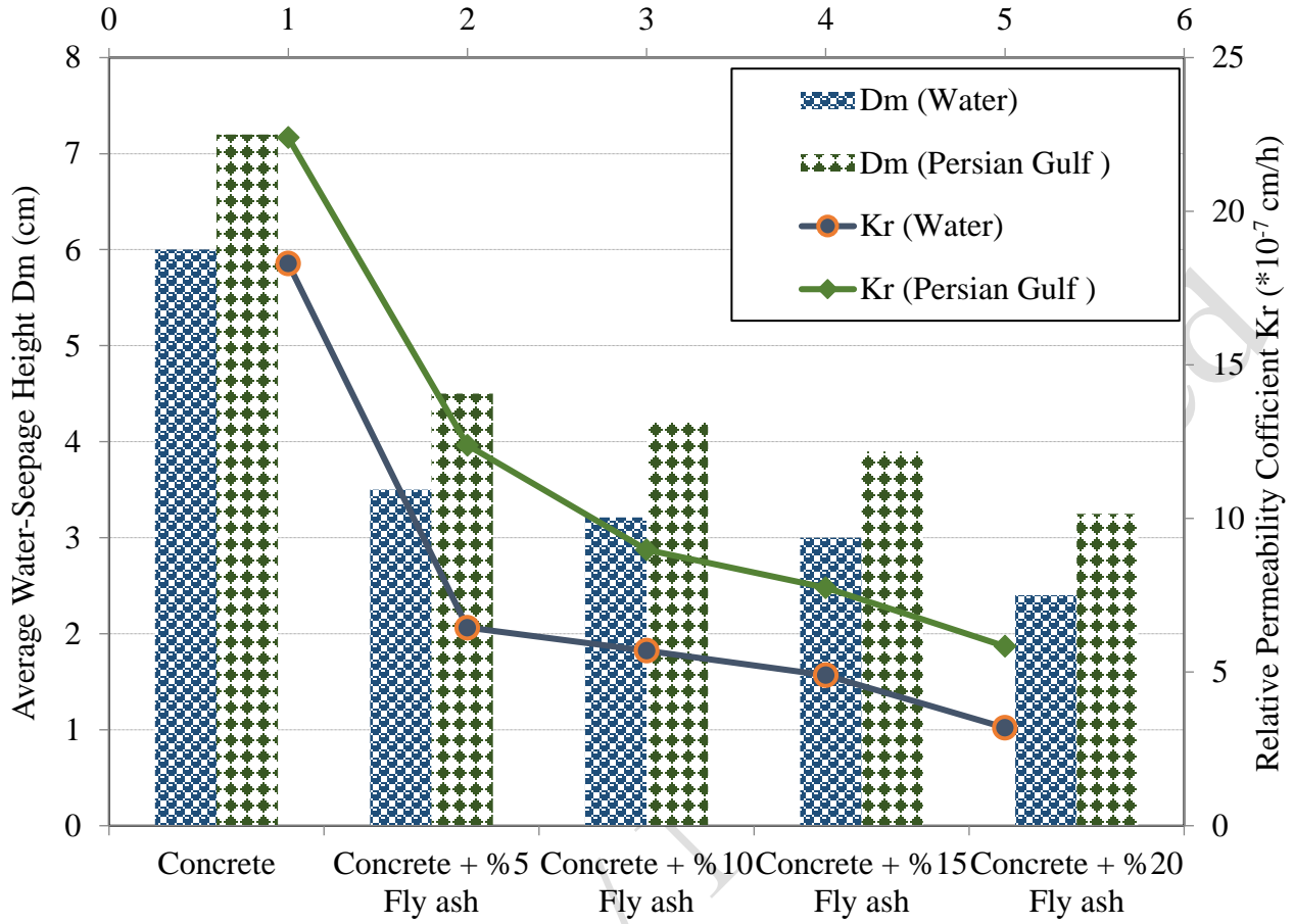
Figure 6: Permeability coefficient and depth of water penetration of concrete samples containing different percentages of fly ash stored in water and the Persian Gulf environment.
