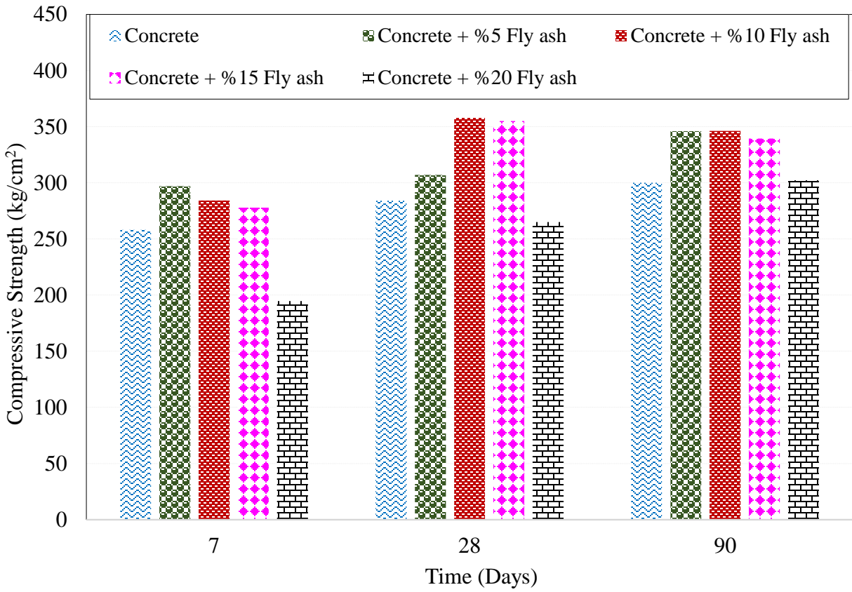
Figure 5: Changes in compressive strength of concrete samples stored in Persian Gulf sea water.
