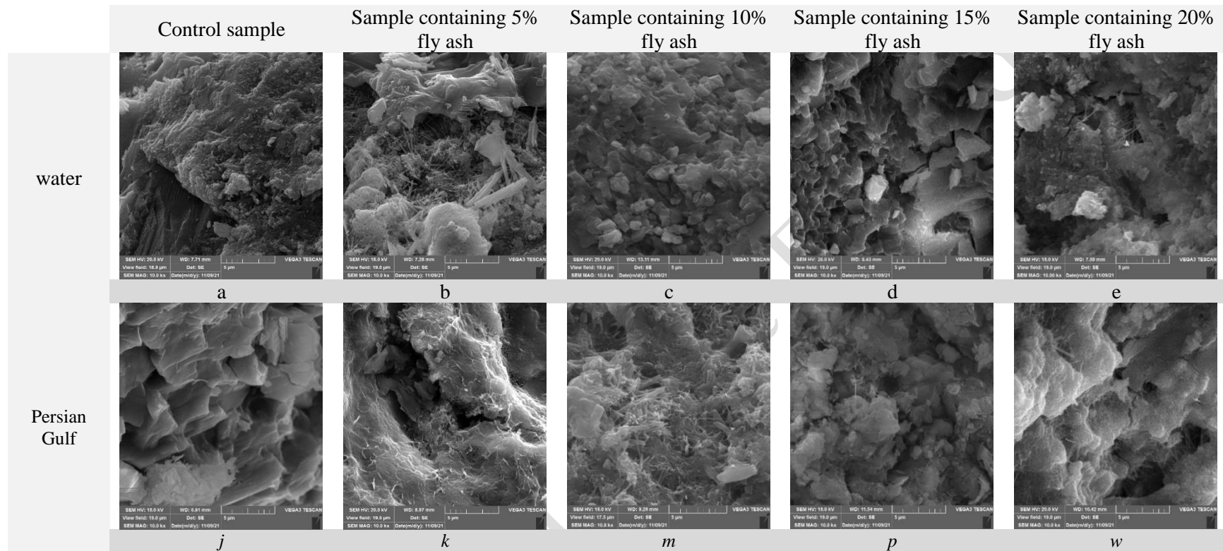
Figure 2: SEM images of concrete samples, including (a) control sample stored in water, (b) sample containing 5% fly ash stored in water, (c) sample containing 10% fly ash stored in water, (d) sample containing 15% fly ash stored in water, (e) sample containing 20% fly ash stored in water, (j) control sample stored in the Persian Gulf, (k) sample containing 5% fly ash stored in the Persian Gulf, (m) sample containing 10% fly ash stored in the Persian Gulf, (p) sample containing 15% fly ash stored in the Persian Gulf, and (w) sample containing 20% fly ash stored in the Persian Gulf.
