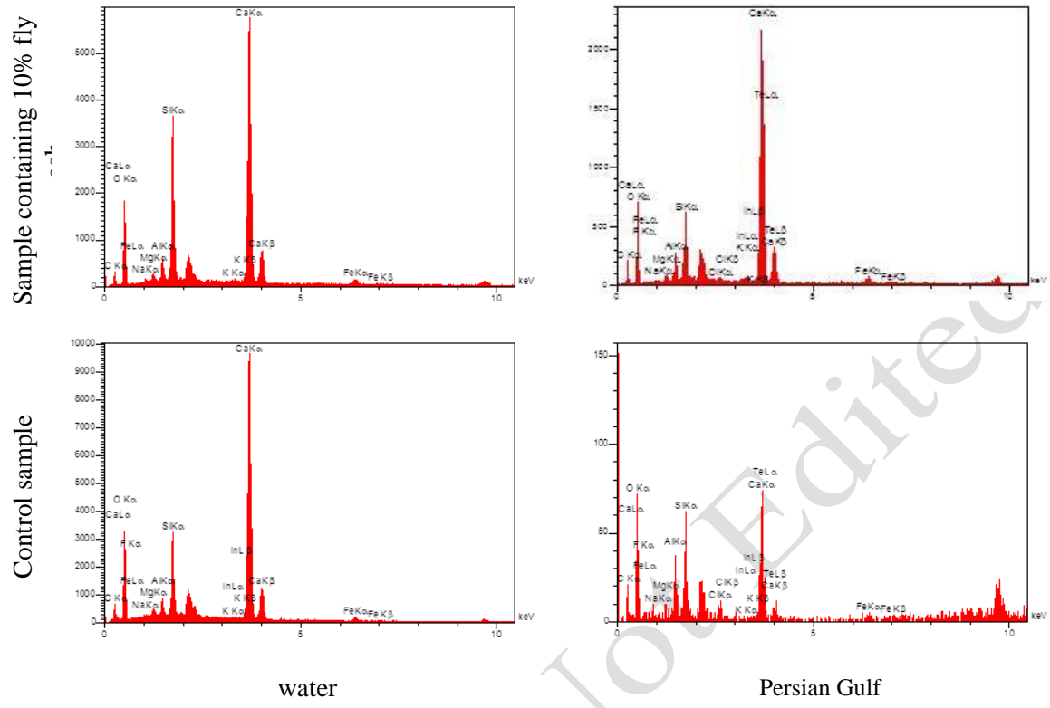
Figure 3: EDX images of concrete samples, including (a) control sample stored in water, (b) sample containing 10% fly ash stored in water, (c) control sample stored in the Persian Gulf, and (d) sample containing 10% fly ash stored in the Persian Gulf.
